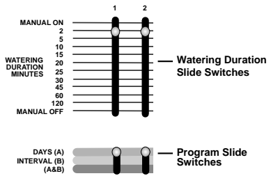
FIGURE 9: Slide Switches
