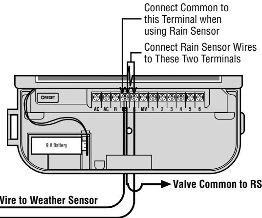
Sensor Wire to Common
